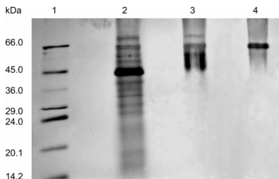
Figure 2. SDS-PAGE (12.5%) of D. hansenii UFV-1 \alpha -galactosidase purification steps. Lane 1, molecular mass standards; lane 2, lyophilized extract fraction; lane 3, Sephadex G-150 fraction; and lane 4, DEAE-Sepharose fraction. Protein gel was stained with silver.
