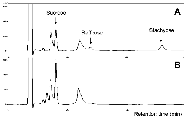
Figure 7. HPLC analysis of hydrolysis products of ROs present in soy milk by extracellular \alpha -galactosidase from D. hansenii UFV-1. (A) Soy milk before enzyme treatment and (B) after 4 h of enzyme treatment.
