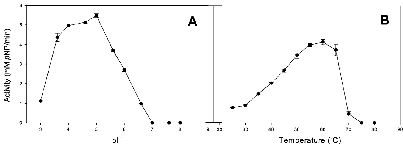
Figure 3. pH (A) and temperature (B) influences on the activity of \alpha -galactosidase from D. hansenii UFV-1.
